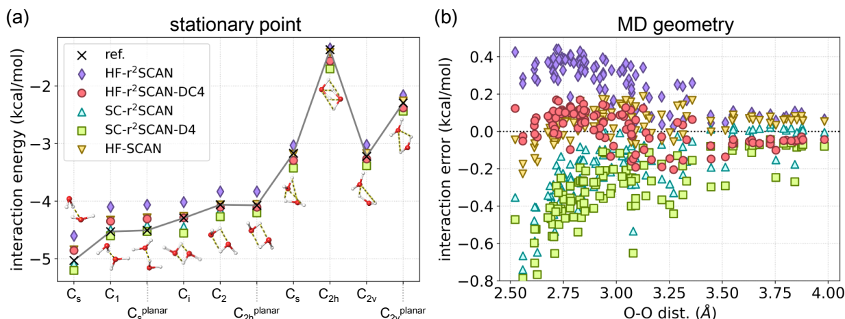
Figure 2. Water dimer interaction energies. (a) Smith stationary points 54 and (b) MD simulated water dimers with the oxygen-oxygen distance. For (a), MAEs of each functional are (following the order in the legend) 0.25, 0.11, 0.09, 0.17, and 0.08 kcal/mol. DLPNO-CCSD(T)-F12 has been used as a reference. For (b), MAE of each functionals are 0.25, 0.08, 0.20, 0.30 and 0.08 kcal/mol. Supplementary Figure 1 shows the corresponding density sensitivities and Supplementary Figure 2 shows the errors of approximations for the Smith dimers and interaction energies for MD dimers.
