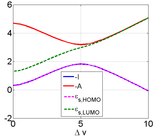
FIG. 12. Plot of -A , -I , \epsilon^{\text{HOMO}} , and \epsilon^{\text{LUMO}} as a function of \Delta v with U = 5 and 2t = 1 .
