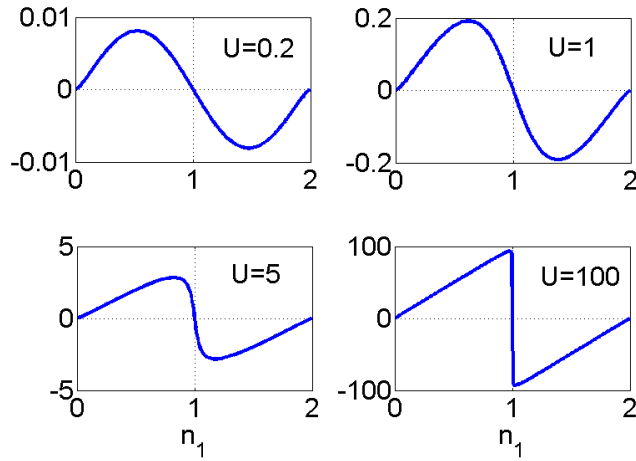
FIG. 10. Plot of \Delta v_C for different U and 2t = 1 .
