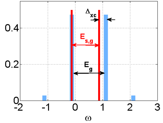
FIG. 13. Spectral function of symmetric dimer for U = 1 , \Delta v = 0 , and 2t = 1 . The physical MB peaks are plotted in blue, the KS in red. Here I = 0.1 , A = -1.1 , and \epsilon^{\text{LUMO}} = 0.9 , corresponding to \Delta v = 0 in Fig. 11.
