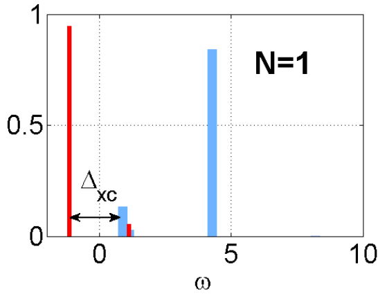
FIG. 18. Spin- \downarrow resolved spectral function for N = 1 and U = 5 , \Delta v = 2 ( 2t = 1 ). Here I = 1.12 , A = -0.90 , and \epsilon^{\text{LUMO}} = \epsilon^{\text{HOMO}} = -1.12 .
