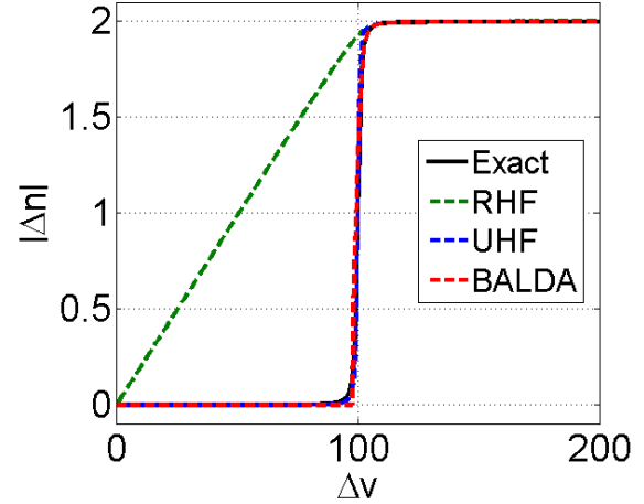
FIG. 32. Plots of \Delta n in HF and BALDA as a function of \Delta v for U = 100 ( 2t = 1 ). The crossover from the charge-transfer to the Mott-Hubbard regime happens at about U \approx \Delta v .
