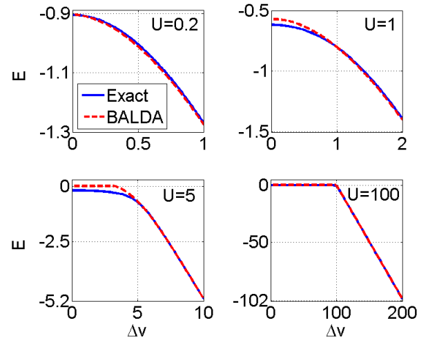
FIG. 26. Ground-state energy versus \Delta v for several U , with 2t = 1 . The BALDA energies are evaluated self-consistently.
