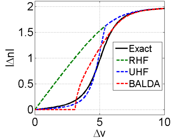
FIG. 24. Plots of \Delta n for HF and BALDA as a function of \Delta v for U = 5 and 2t = 1 . The crossover from the charge-transfer to the Mott-Hubbard regime happens at U \approx \Delta v .
