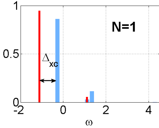
FIG. 17. Spin- \downarrow resolved spectral function for N = 1 and U = 1 , \Delta v = 2 , ( 2t = 1 ). Here I = 1.12 , A = 0.27 , and \epsilon^{\text{LUMO}} = \epsilon^{\text{HOMO}} = -1.12 .
