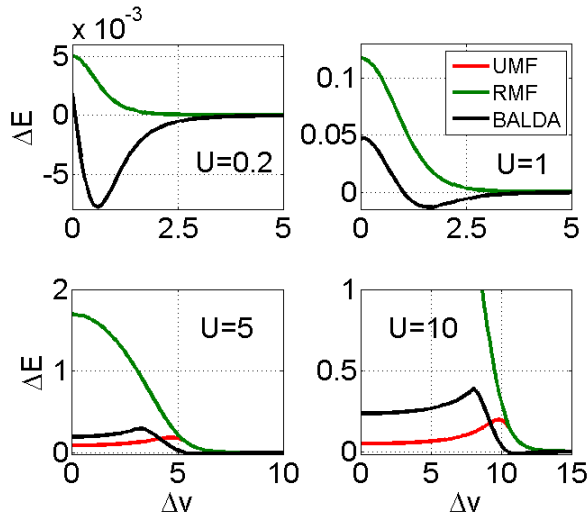
FIG. 27. Plots of the RMF, UMF, and BALDA \Delta E = E^{\text{approx}} - E^{\text{exact}} as a function of \Delta v for U = 0.2, 1, 5 , and 10 . For small U the RMF and UMF results are indistinguishable. Here 2t = 1 .
