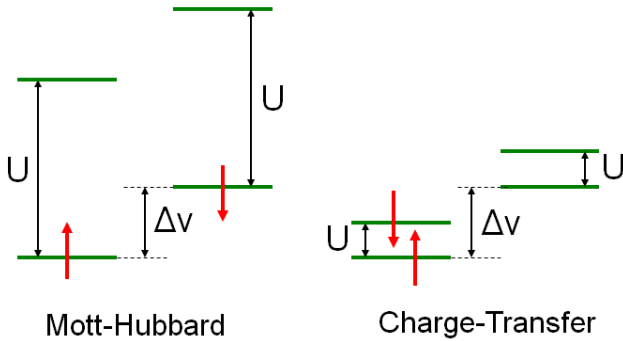
FIG. 1. Many-body view of two distinct regimes of the asymmetric Hubbard dimer. On the left, the charging energy is much greater than the difference in on-site potentials. On the right, the situation is reversed.
