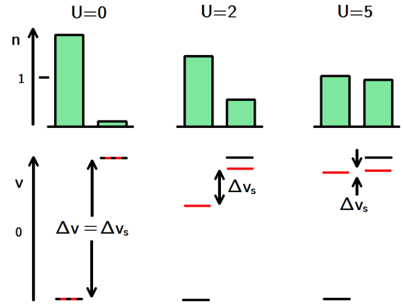
FIG. 2. DFT view: occupations n and potentials v of an asymmetric half-filled Hubbard dimer as a function of U . The on-site potential difference \Delta v is shown in black and the KS on-site potential difference \Delta v_s is in red. The second and third panels correspond to the situations of Fig. 1.
