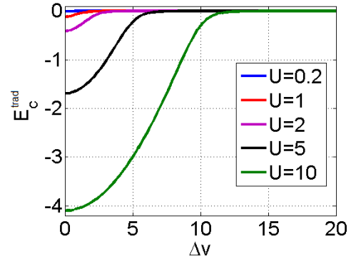
FIG. 6. Correlation energy E_{\text{C}}^{\text{trad}} of Hubbard dimer as a function of \Delta v for several values of U and 2t = 1 .
