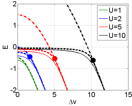
FIG. 25. Ground-state energy of the unrestricted Hartree-Fock (thick dashed line), restricted Hartree-Fock (dot dashed line), and exact ground-state (thin solid line) of the Hubbard dimer as a function of \Delta v for several values of U and 2t = 1 . The dot shows the Coulson-Fischer point at which the symmetry breaks spontaneously. For smaller \Delta v the UHF energy is below RHF while for larger \Delta v they are the same.
