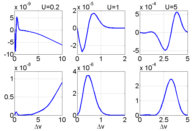
FIG. 23. Top row: Error in density as a function of \Delta v . Bottom row: Error in ground-state energy as a function of \Delta v and 2t = 1 .
