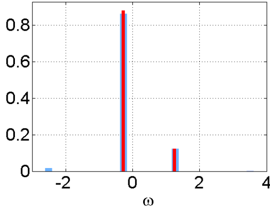
FIG. 15. Same as Fig. 13, but now U = 1 , \Delta v = 2 . Here I = 0.27 , A = -1.27 , and \epsilon^{\text{LUMO}} = 1.25 , corresponding to \Delta v = 2 in Fig. 11.
