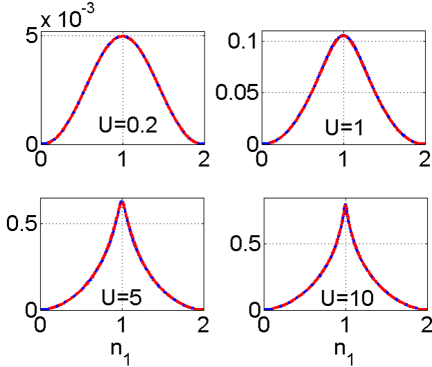
FIG. 19. Plot of exact T_C (blue line) and T_{C,\text{par}} (red dashed line) for different U and 2t = 1 .
