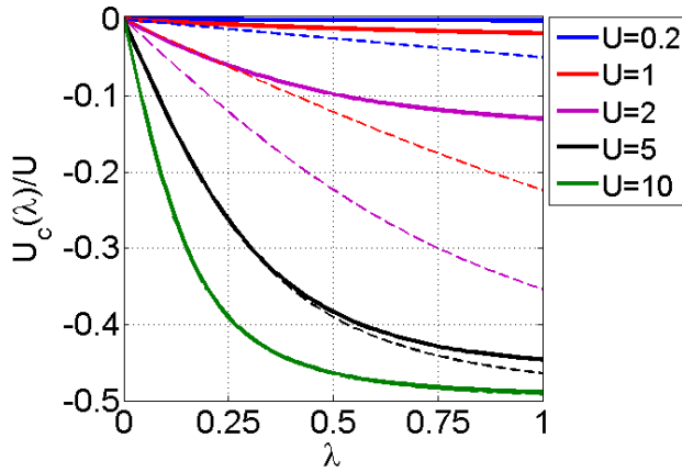
FIG. 21. Adiabatic connection integrand divided by U for various values of U . The solid lines are \Delta v = 2 and the dashed lines \Delta v = 0 . Asymmetry reduces the correlation energy but increases the fraction of kinetic correlation.
