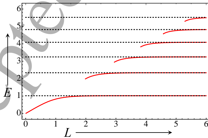
42 43 44 45 46 47 48 49 50 51 52 53 54 55 56 57 58 59 60 Figure 2. Red curves: even and odd energy levels in the truncated potential (1.2), for increasing truncation distance L ; dotted lines: levels of the untruncated linear potential, i.e. zeros of Ai' (even levels) and Ai (odd levels).
