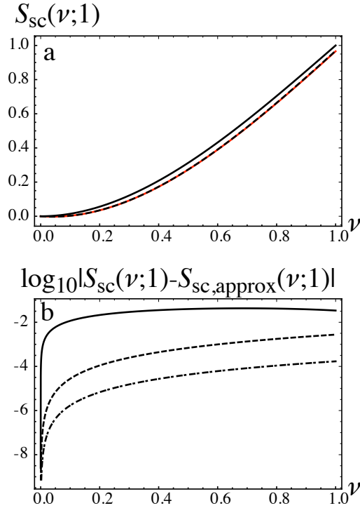
Figure 2. Energy sums for Pöschl-Teller potential for D=1 . (a) The full red curve (colour online) is the exact scaled sum S_{\text{sc}} from (5.3) and (5.4); the full black curve is the leading approximation S_{\text{sc}0} in (5.5), and the dashed black curve (visually indistinguishable from the exact sum) is the next approximation S_{\text{sc}1} . (b) Errors S_{\text{sc}} - S_{\text{sc,approx}} , where S_{\text{sc,approx}} = S_{\text{sc}0} (full curve), S_{\text{sc,approx}} = S_{\text{sc}1} (dashed curve), and S_{\text{sc,approx}} = S_{\text{sc}2} (dot-dashed curve)
