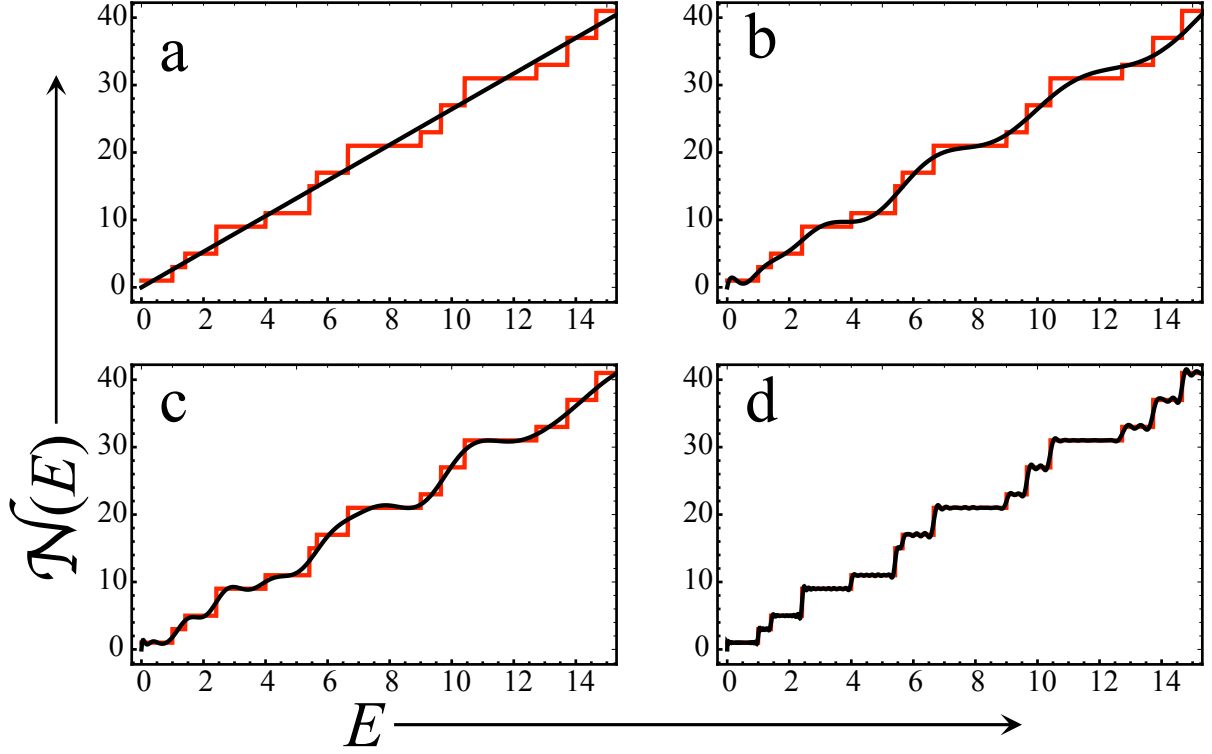
Figure 4. Staircase function (7.5) for \alpha=1/2^{1/4} , including periodic orbits with |j|, |k| \leq K , where (a) K=0 , (b) K=1 , (c) K=2 , (d) K=20 ; stepped curves (red online): exact stair; black curves: approximate stairs
