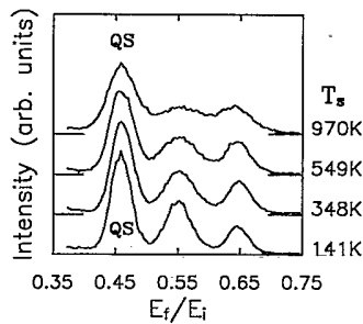
FIG. 1. Typical measured energy spectra for 201.2 eV \text{Na}^+ scattering from Cu(001) as a function of surface temperature. The beam was incident along the \langle 100 \rangle azimuth, with \theta_i = \theta_f = 45^\circ . The peak labeled QS is due to a quasisingle collision with a Cu atom (see text).
